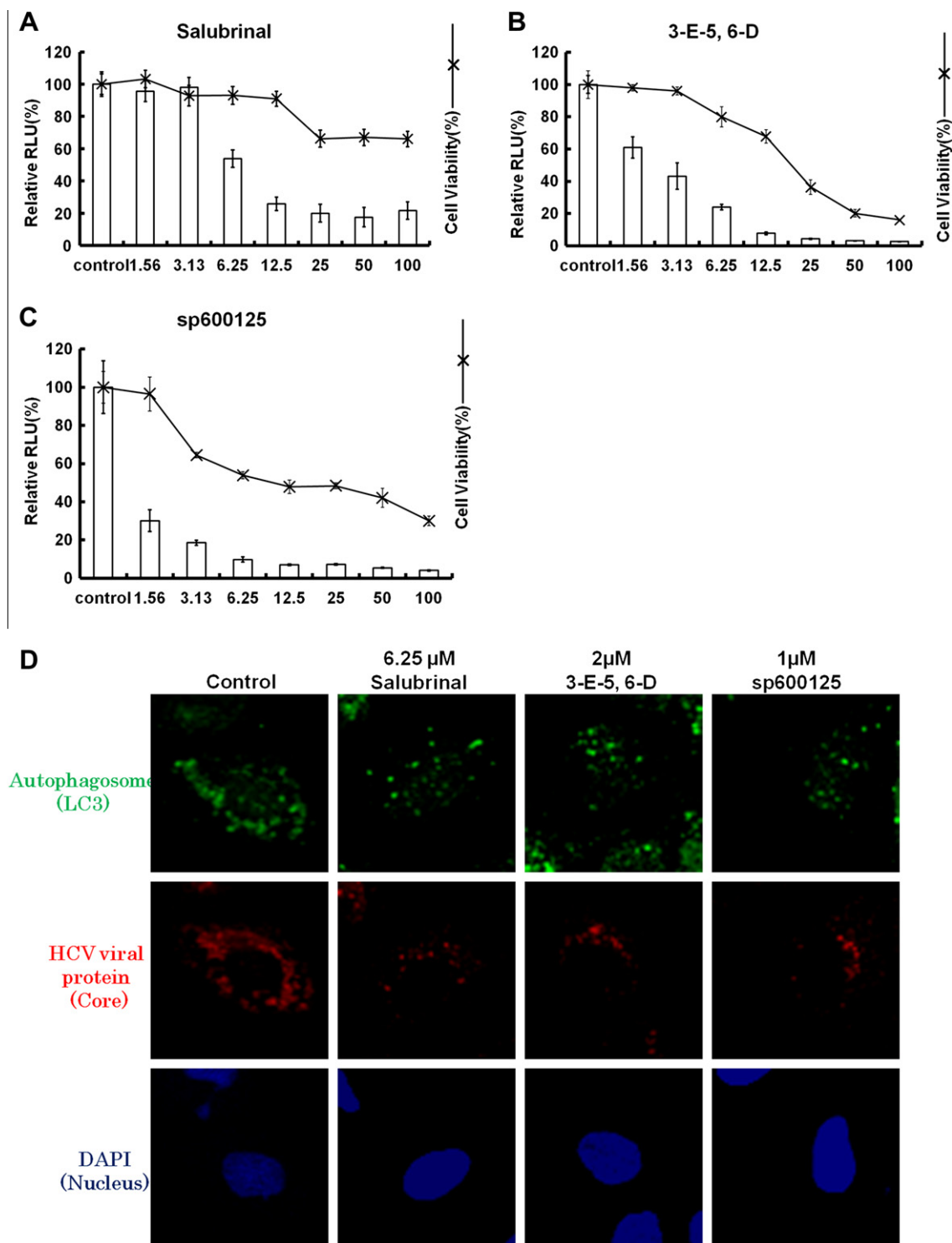
Fig. 3. Regulation of HCV replication by inhibitors of UPR. The effects of Salubrinal (eIF2- \alpha phosphatase inhibitor), 3-E-5, 6-D (XBP-1 splicing inhibitor) and sp600125 (JNK inhibitor) on HCV replication in the OR6 assay system were examined. OR6 cells were treated with Salubrinal (A), 3-E-5, 6-D (B) or sp600125 (C) inhibitor for 72 h, following which the RL assay (bar graph) and WST-1 assay (line graph) were performed. The relative values (%) calculated at each point, with the level in the non-treated cells set at 100%, are presented here. (D) fluorescence microscopy. Green: LC3 staining of the autophagosomes; blue: DAPI staining of the nuclei; red: staining of the HCV core protein.
